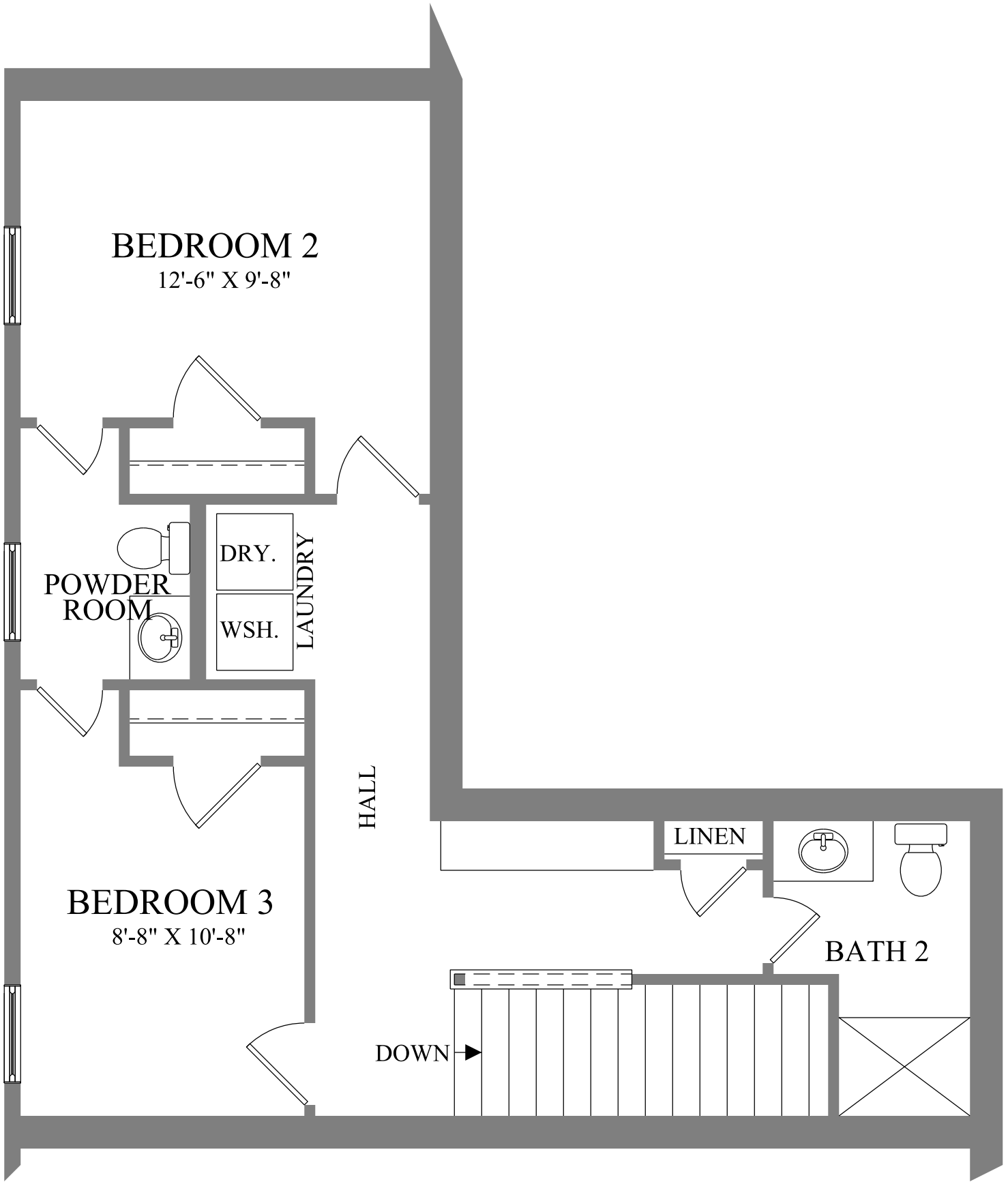
SMYTH COURT 3 BEDROOM TOWNHOUSE SECOND FLOOR PLAN
