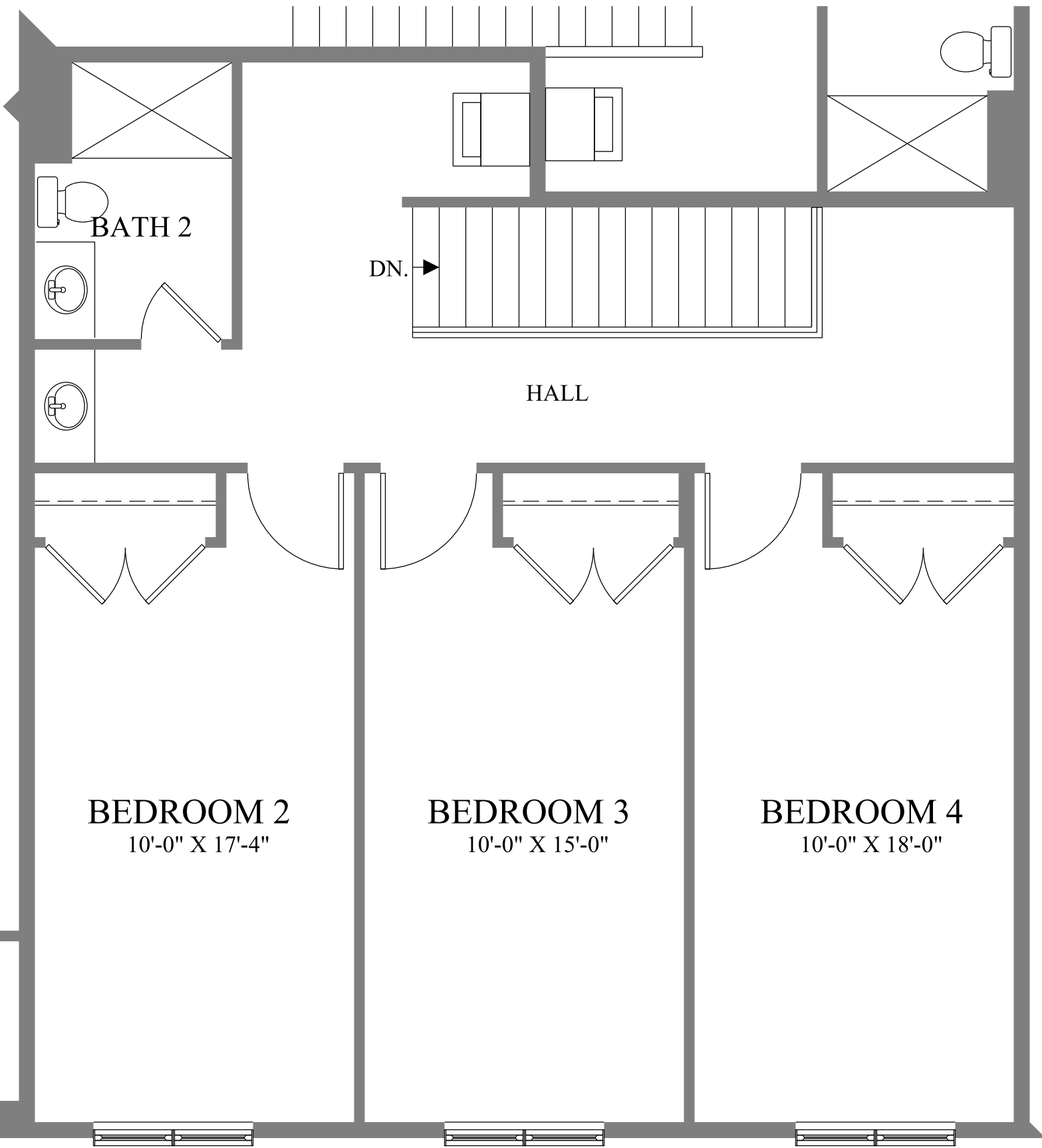
119 SOUTH MAIN STREET 4 BEDROOM INTERIOR REAR VIEW APARTMENT SECOND FLOOR PLAN
